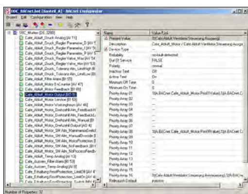
BACnet configurator
