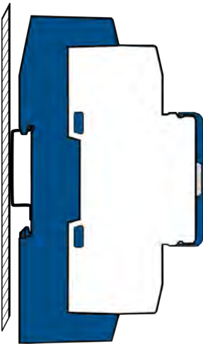
on DIN rails 35 mm (in accordance with DIN EN 60715) TH35
