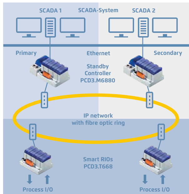
Typical layout of a redundancy system with two PCD3.M6880 Standby devices and PCD3.T668 Ethernet Smart RIOs.
