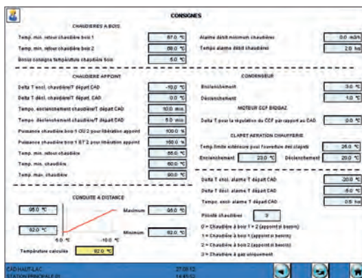
▲ Instructions on the web panel
