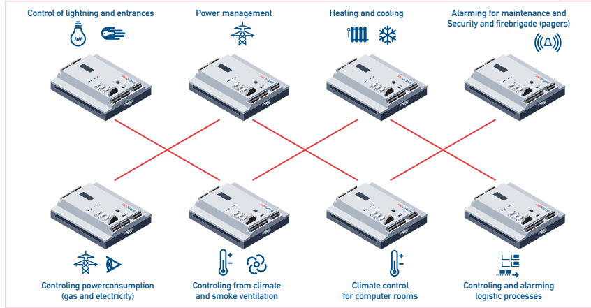
A total of 140 CPUs PCD2.M170. All conected through separate Ethernet for building automation
