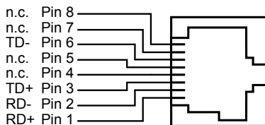
Fig. 2: Pin configuration of aTP interface
