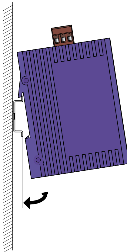
Fig. 5: Assembling
