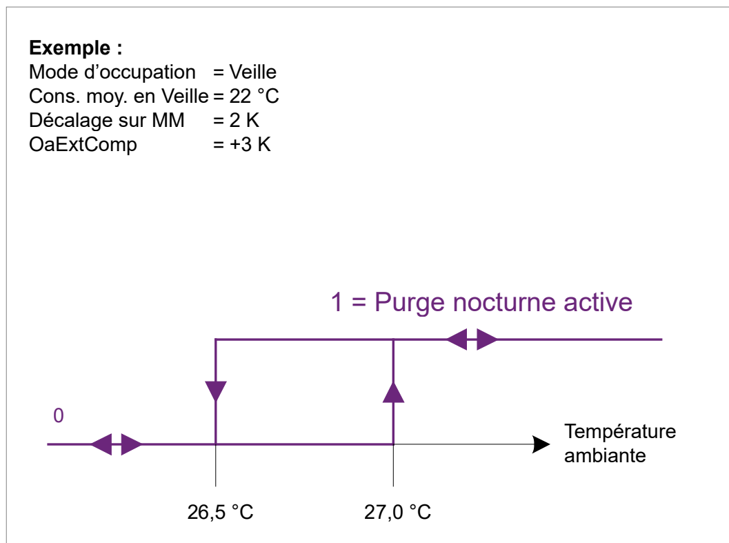
Image 20. Purge nocturne
