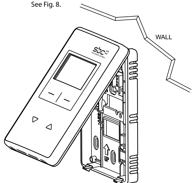
Fig. 8. Removing Wall Module from Subbase.
