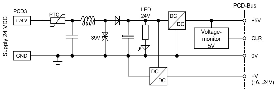
Terminals for power supply 24 VDC
