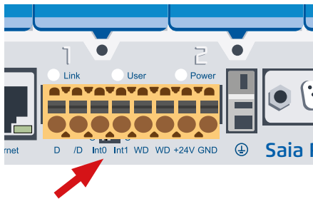
Terminal 3 and 4 for interrupts inputs Int0 and Int1
