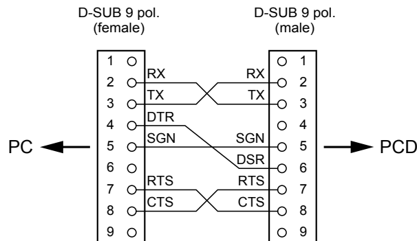
Connection cable PCD8.K111
