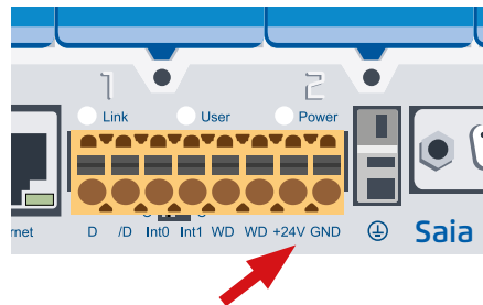
Terminals for power supply 24 VDC
